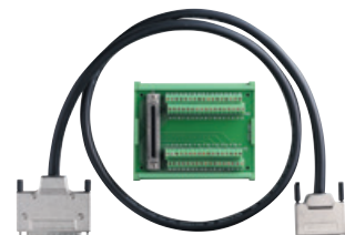
Termination board DIN-68S/1M
